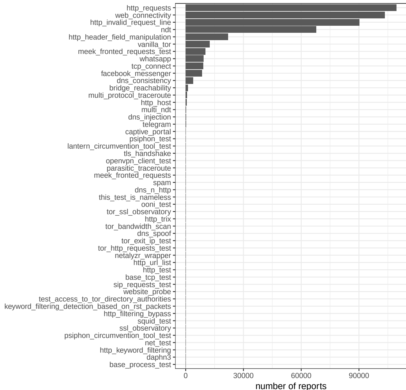
Number of OONI reports by test name
