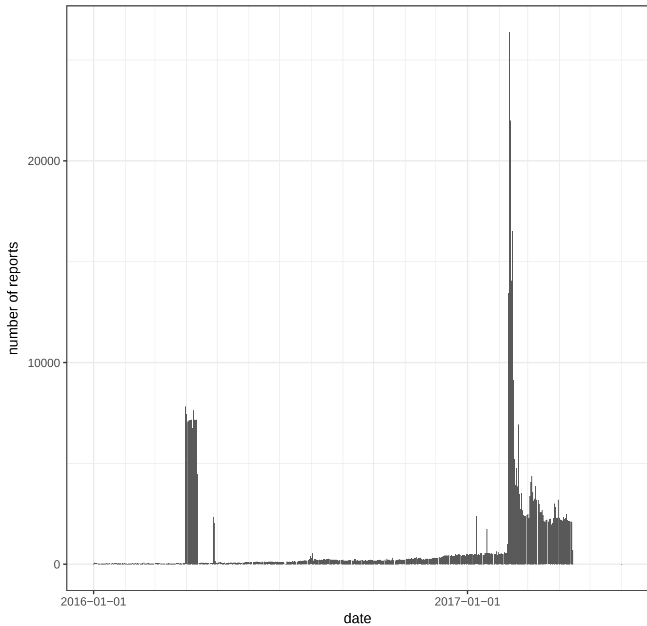
Number of OONI reports per day
