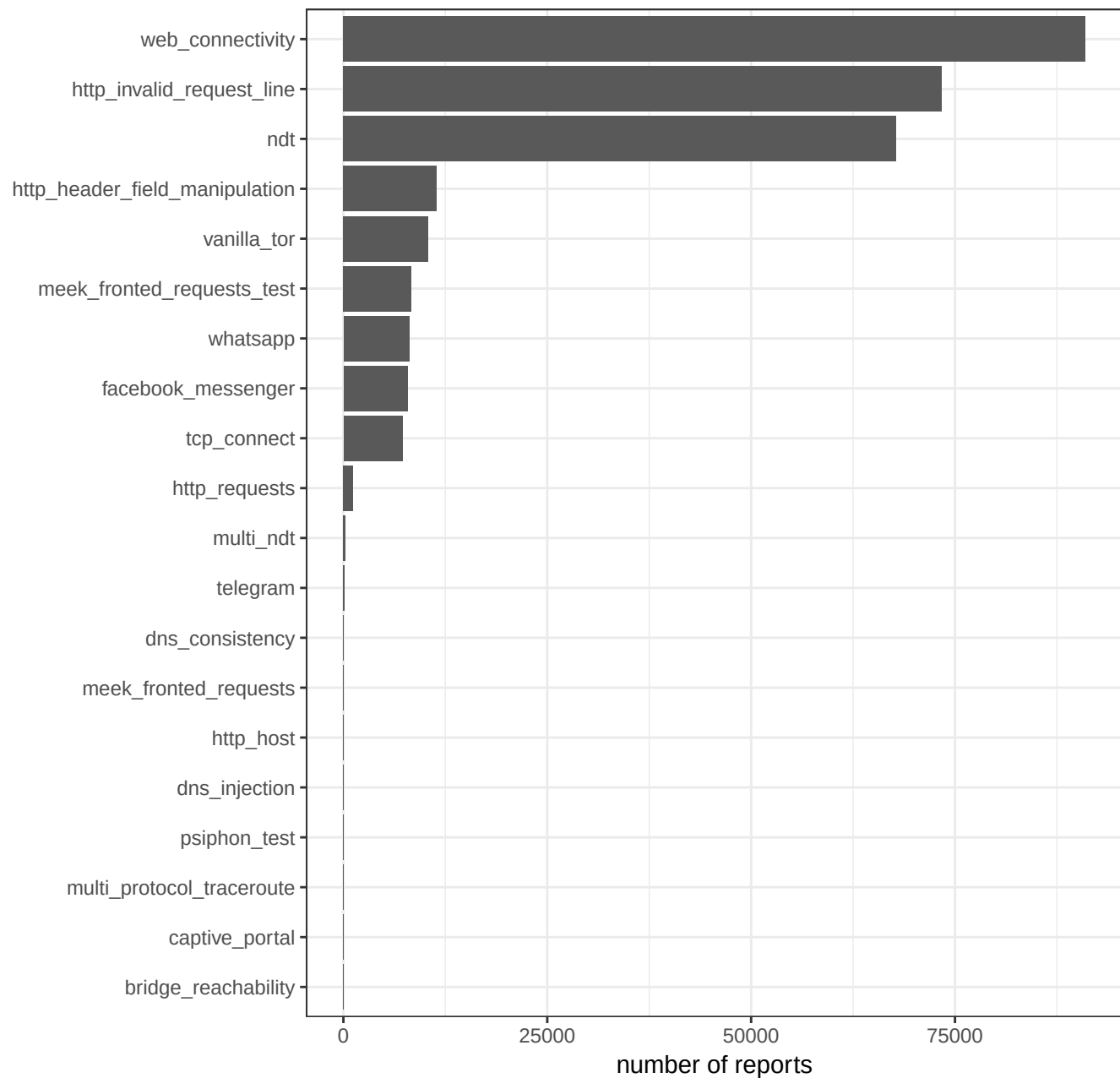
Number of OONI reports by test name (since 2017-01-01)
