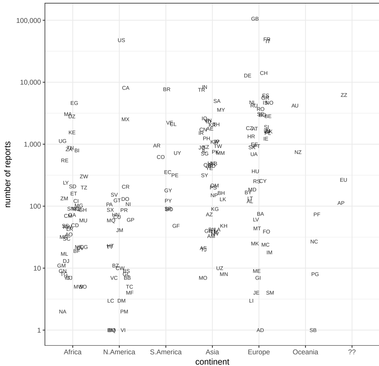
Number of OONI reports by country and continent
